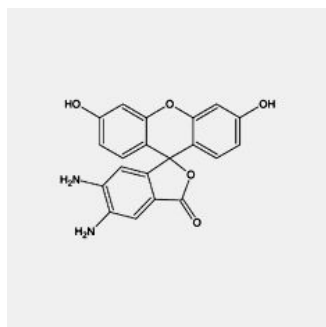
Structure of DAF-2
