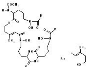
structure of Desferricoprogen Struktur von Desferricoprogen
