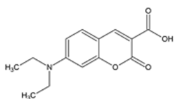
Structure of DEAC (acid)
